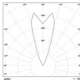
Tube S 1GU10 O15 UP
