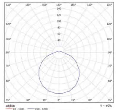
Pollux B 132 H42
