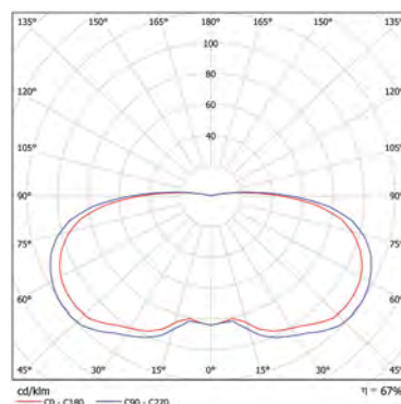
Sphere 150 H97 CLR RFL
