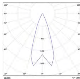
Tube S 1GU10 O14 DOWN
