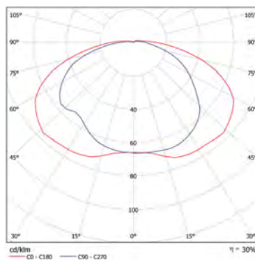
Oval 118 Q84 HF
