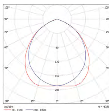
Orion 218 B27 SOP HF
