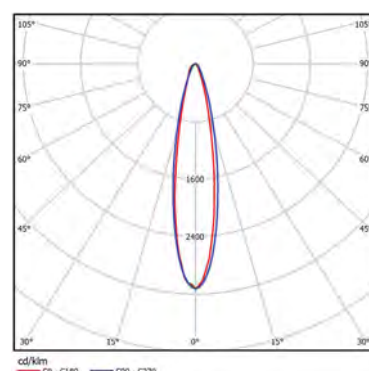
Arena 11000 N87 SPOT
