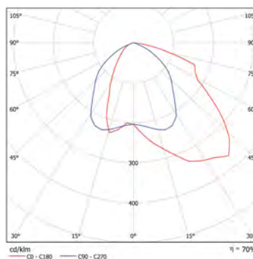
Boreas 1250 K55 CL HI
