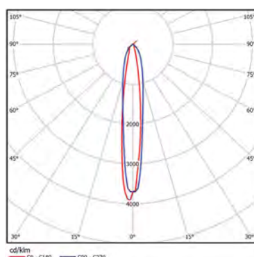
Arena 11000 N87 SPOT BLD
