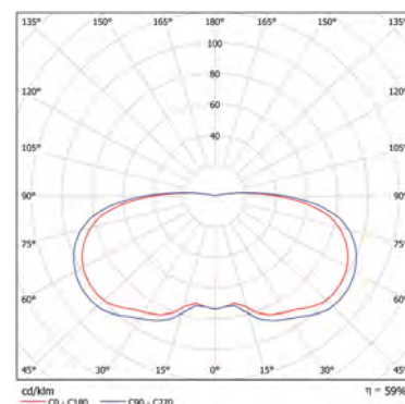
Cylinder 150 H99 CLR RFL PC
