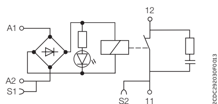
RB(R)101R-24VUC
