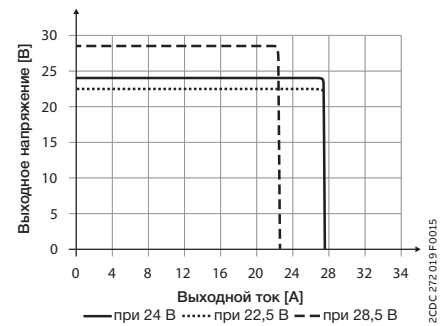
CP-C.1 24/20.0
