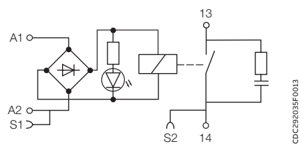
RB(R)111R-24VUC
