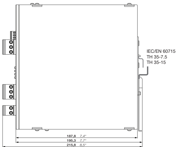
CP-B 24/20.0
