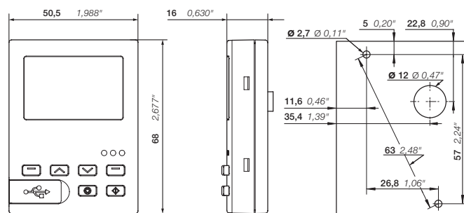
UMC100.3-PAN
